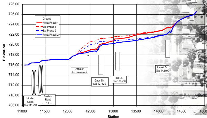
Phase 1 & 2 Improved Water Surface Profile 100-yr
